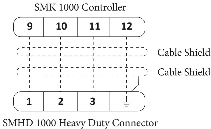
Figure 8 : Wiring diagrams
