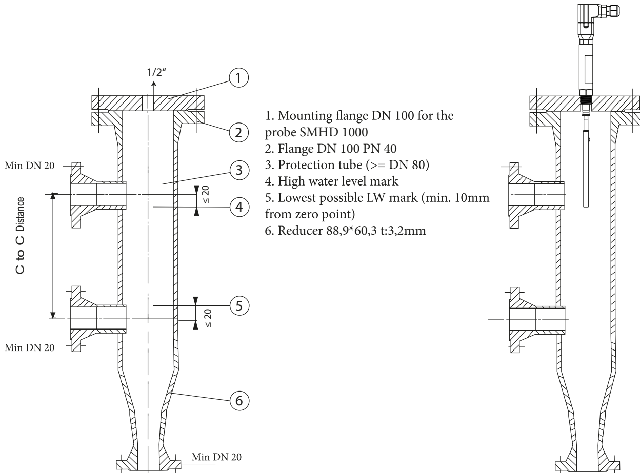
Figure 5 : Installation example 3, usage with protection tube outside the boiler.
