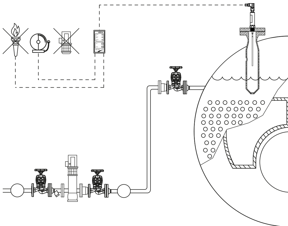
Figure 1 : SMH 1000 System Application
