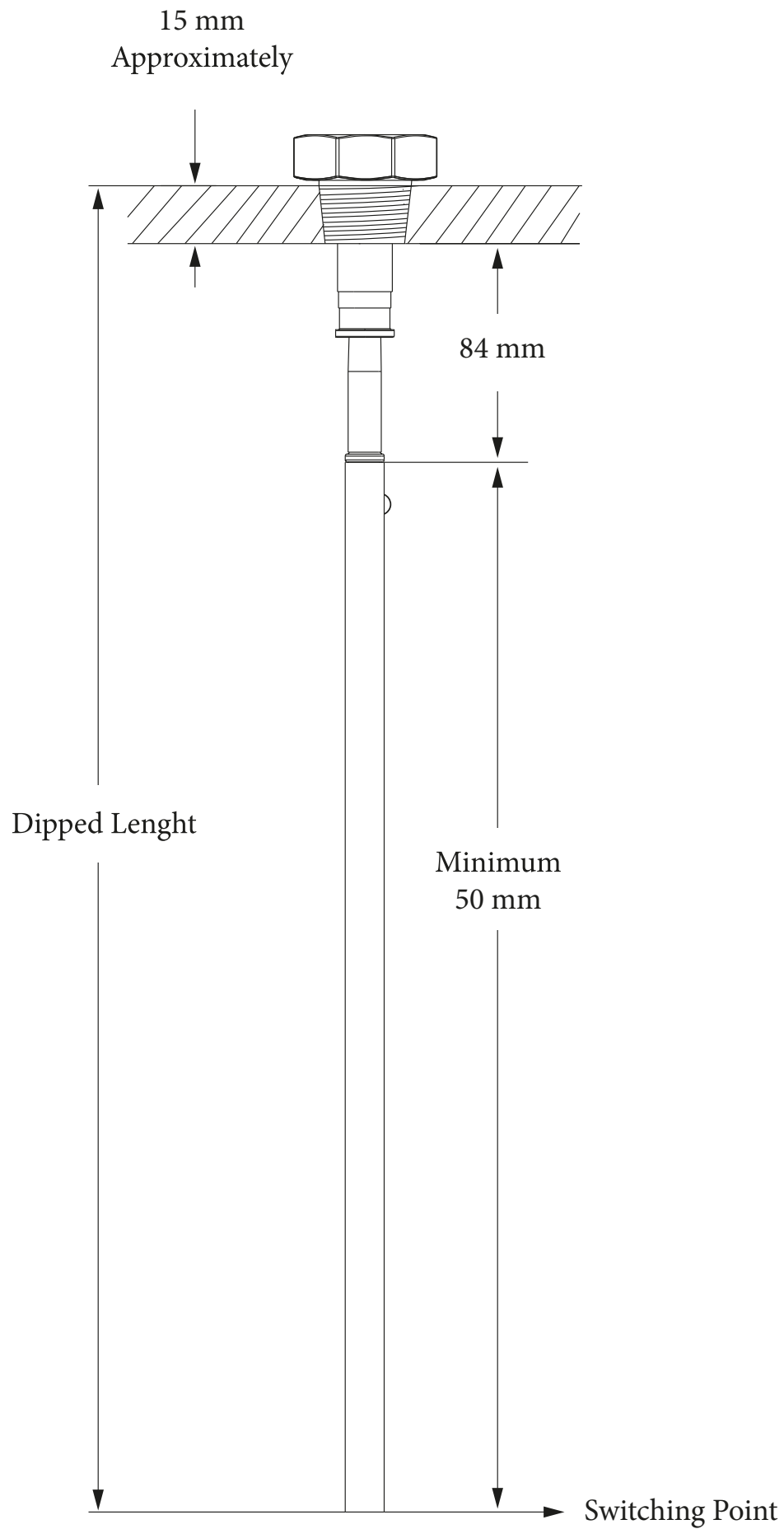
Figure 6 : SMHD 1000 Probe length indication.
